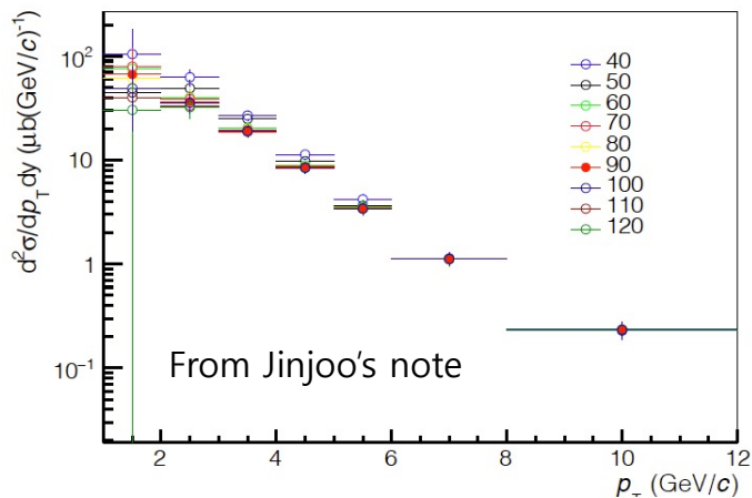
Fig. D.2: The cross section for each opening angle cut.
